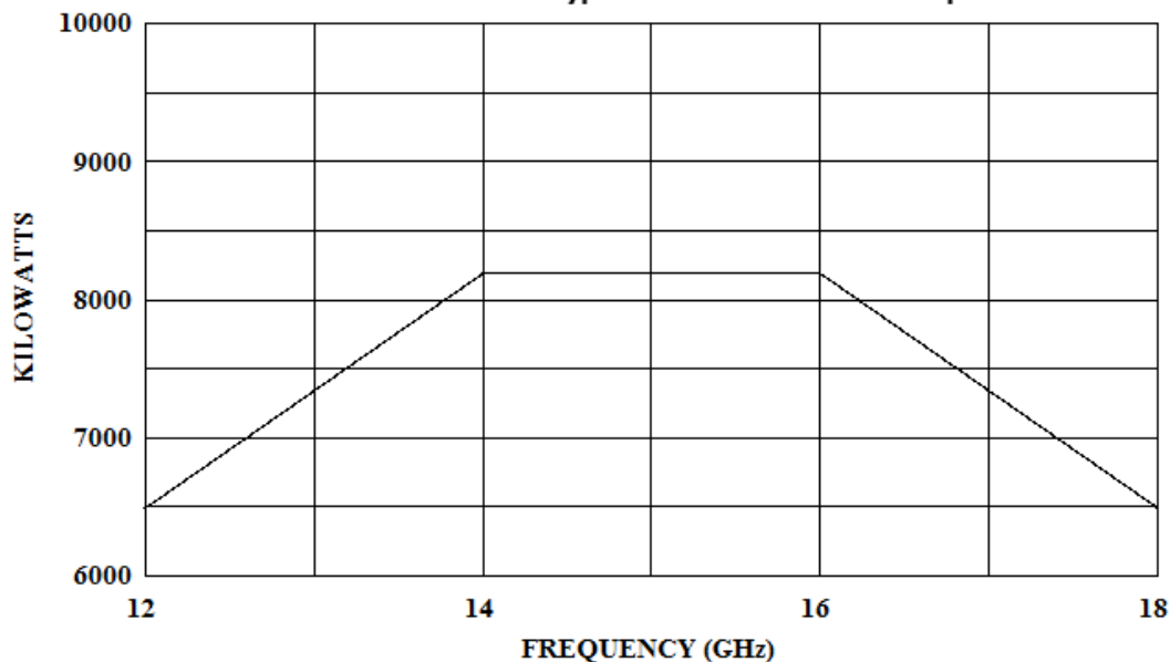
Model 5700TP12G18 Typical Peak Pulse Power Output
